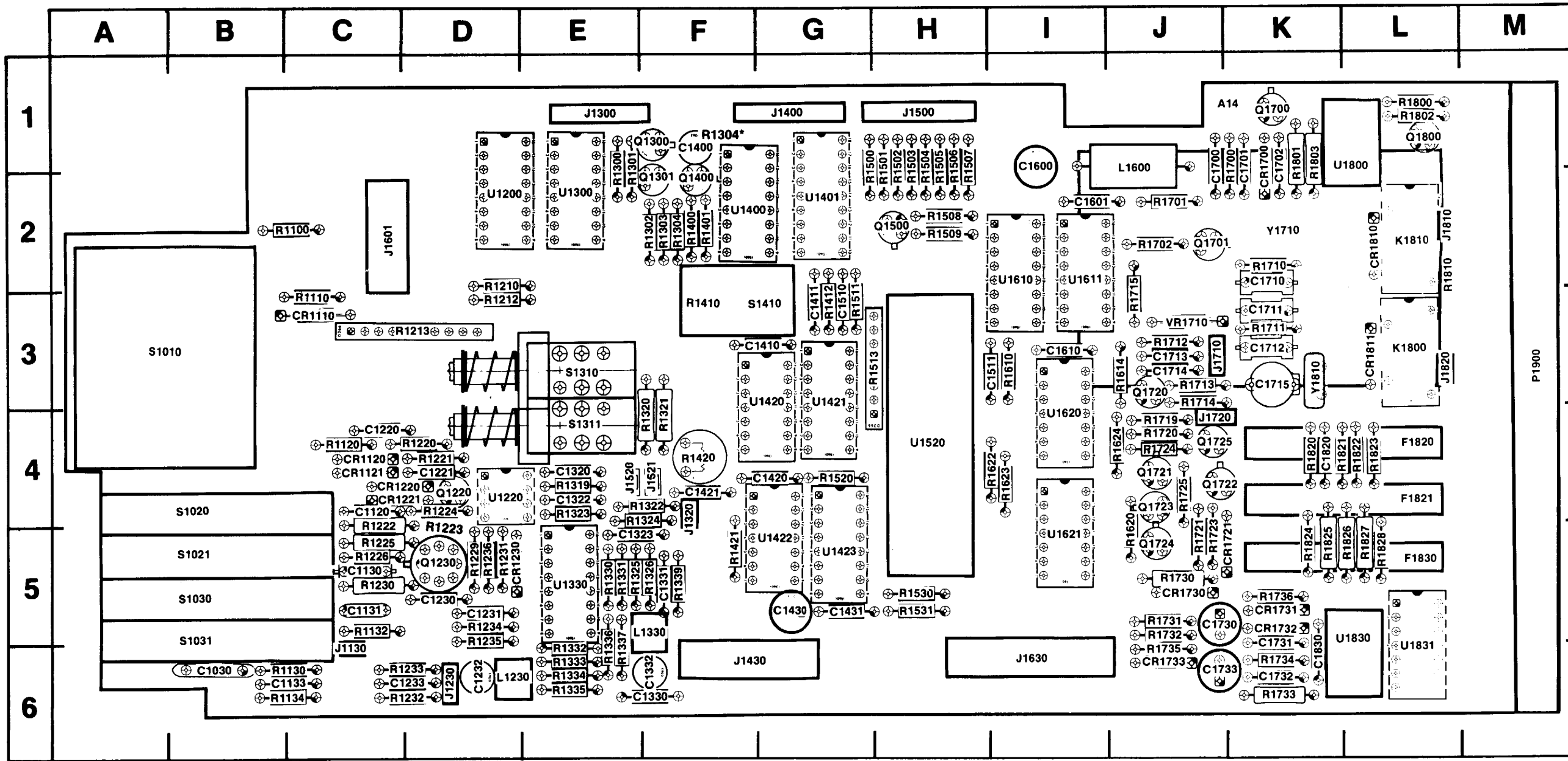
Fig. 8-4. Main Board (A14 Assy).
