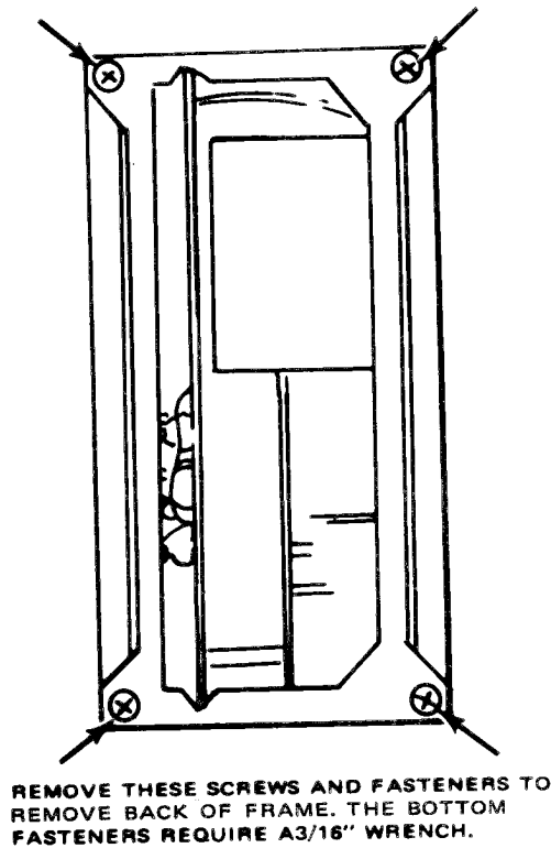
Fig. 5-6. Rear frame removal.
